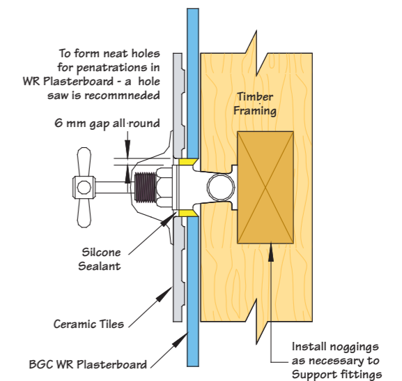
Figure 3 - Sealing Penetrations
